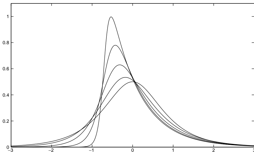
Figure 1 A family of probability density curves with fixed mean and variance, and varying skewness. As the skewness increases, the bulk of the density shifts negatively.
