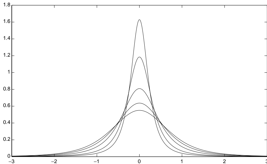
Figure 2 Family of probability densities with fixed mean, variance, and skewness. The kurtosis is different for each curve, and the most leptokurtotic distribution has the sharpest peak in the center.
