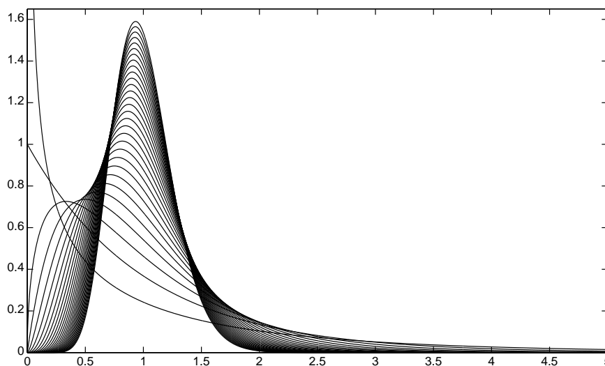
Figure 3 A family of scaled chi-squared distributions. This family arises as the distribution of variances in normal models. The family begins as a highly skewed non-normal distribution and has a bell-shaped normal curve as its limit.
